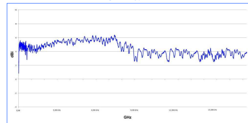
Gain Diagram HyperLOG 30180
