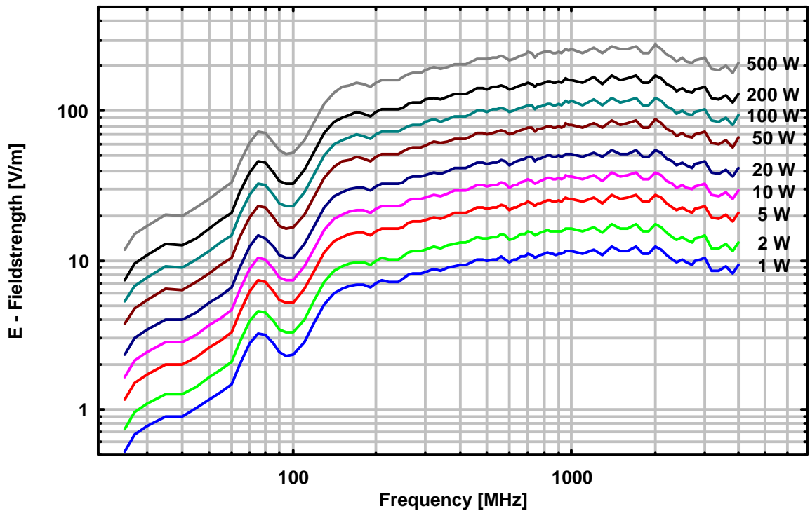
VULB 9163 Generated Fieldstrength 2 m Tip - EuT
