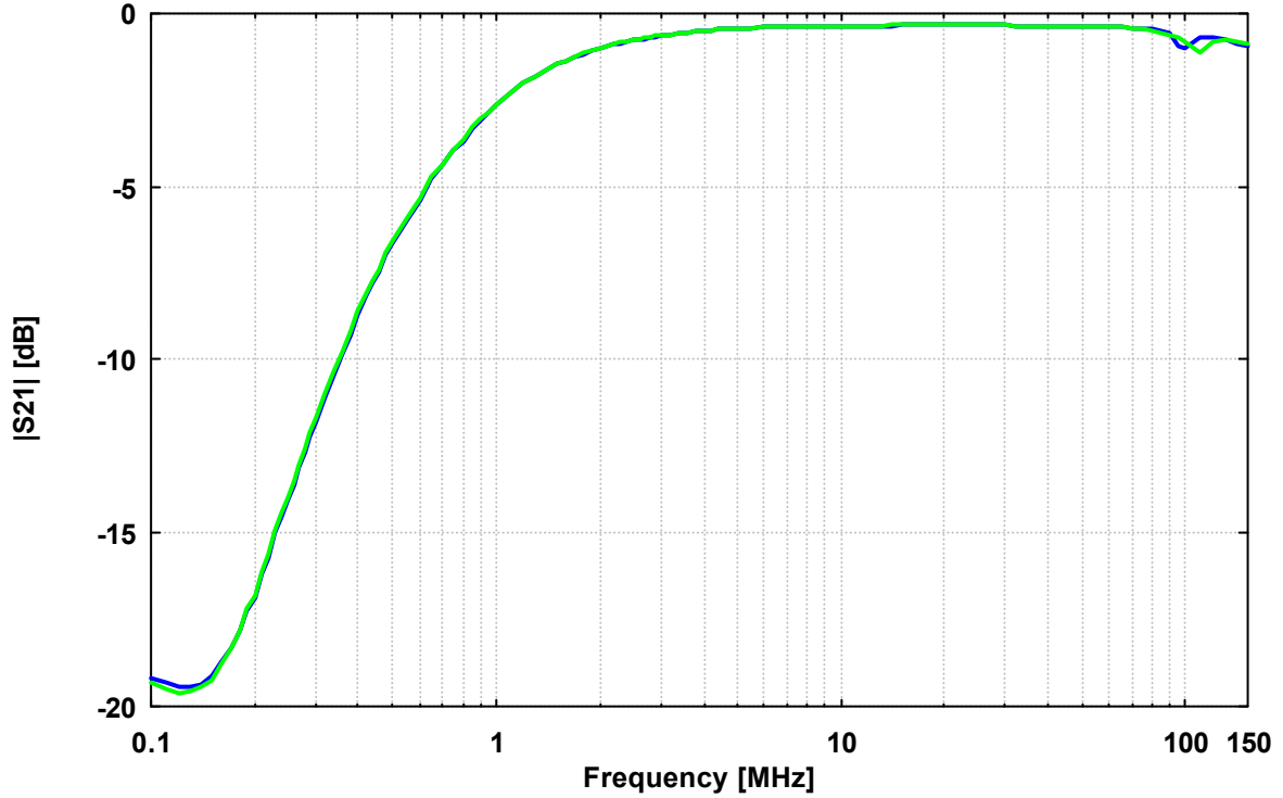
Measured Attenuation EuT-Terminals to BNC (Adapter required)
